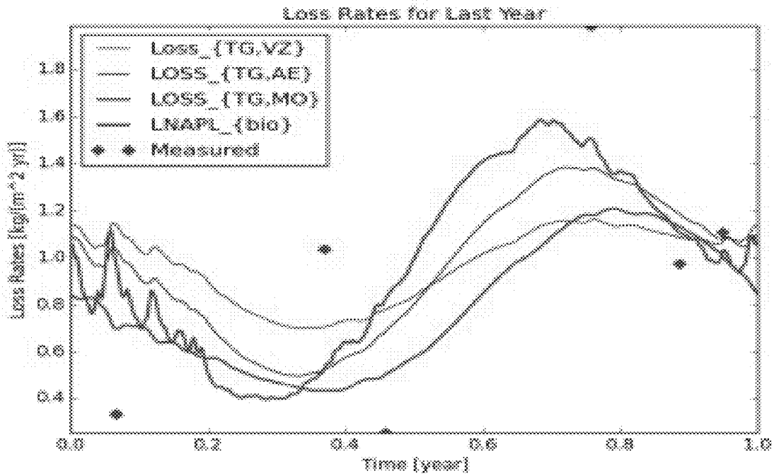
Figure 7: Background corrected estimated and modeled LNAPL loss rates for Bemidji using daily ambient temperatures from a nearby weather station
