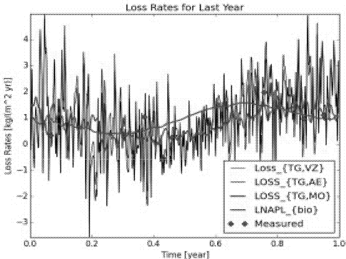
Figure 8: Background corrected estimated and modeled LNAPL loss rates for Bemidji LNAPL loss estimations for the Bemidji site, compared to modeled and field measured LNAPL losses, using daily ambient temperatures from a nearby weather station. The background correction was assumed to have a different thermal conductivity ( k = 0.8 \text{ J/m/K/s} , instead of the original k = 0.7 \text{ J/m/K/s} for the impacted area site).
