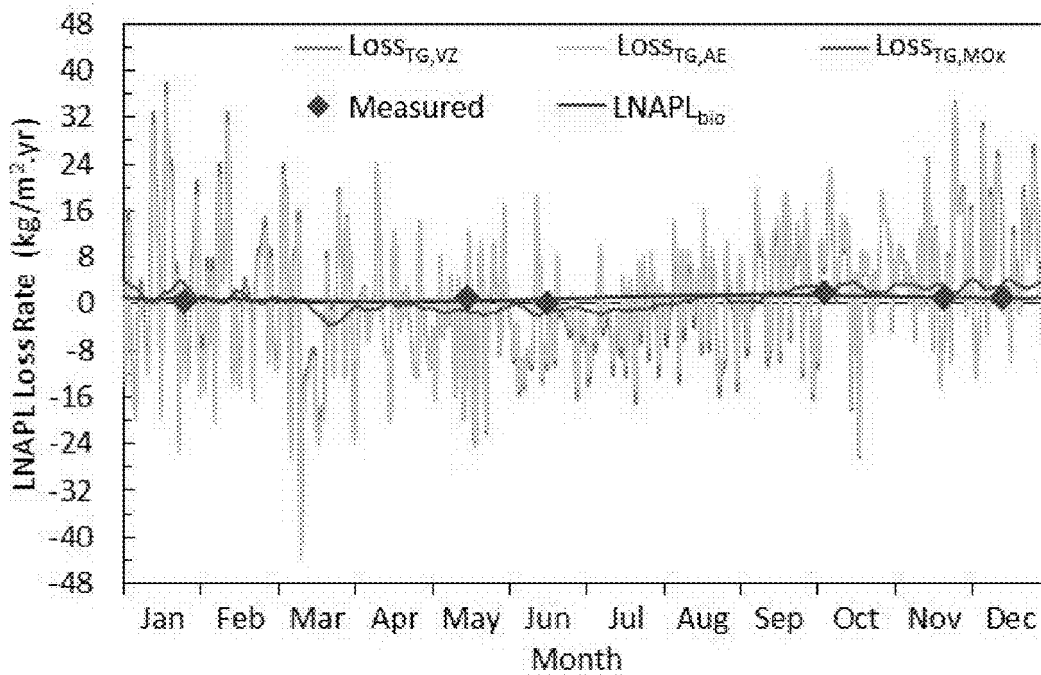
Figure 6: LNAPL loss estimations for the Bemidji site, compared to modeled and field measured LNAPL losses, using daily ambient temperatures from a nearby weather station.
